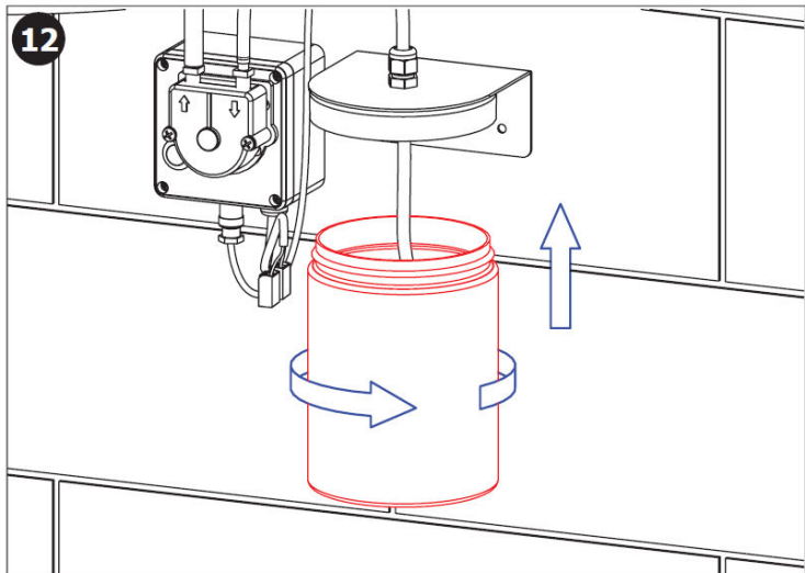
Screw soap canister into top plate
