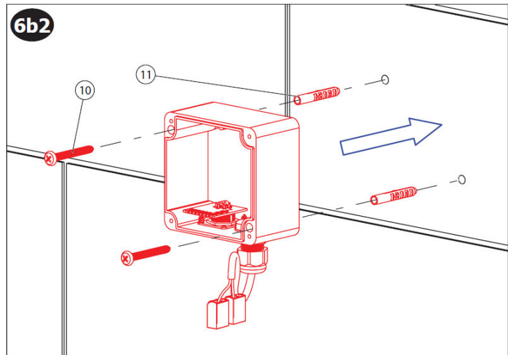
Mark mounting points on surface, drill and insert appropriate wall anchors if required, fix mounting box to wall
