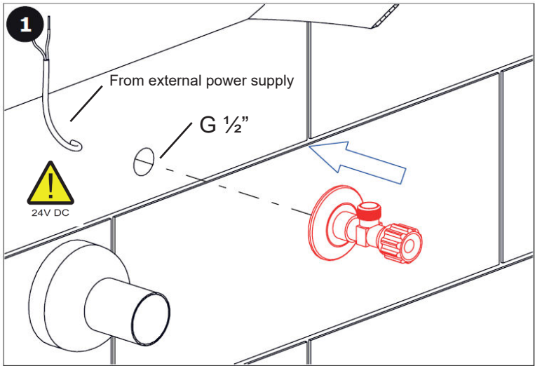
Install 1/2" angle valve (not supplied)
