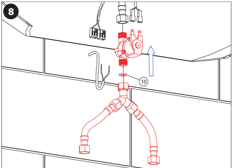
Fit remaining connection hose, washer and solenoid. Note arrow on solenoid valve for water flow direction
