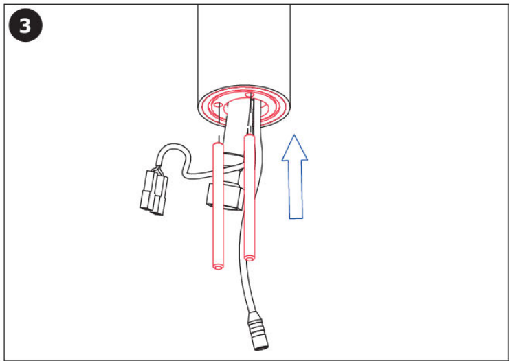
Fit mounting screws, o-ring and rubber gasket
