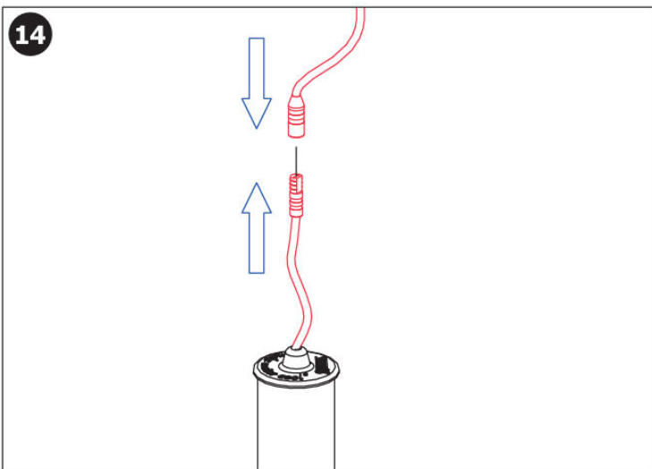
Connect battery to faucet by aligning guide lines on respective cables
