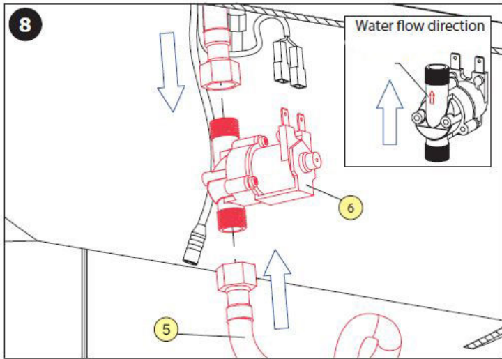
Fit remaining connection hose and solenoid. Note arrow on solenoid valve for water flow direction
