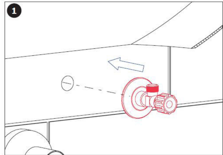
Install 1/2" angle valve (not supplied)
