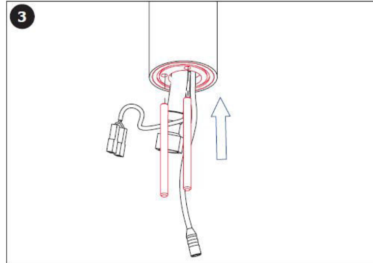
Fit mounting screw, o-ring and rubber gasket
