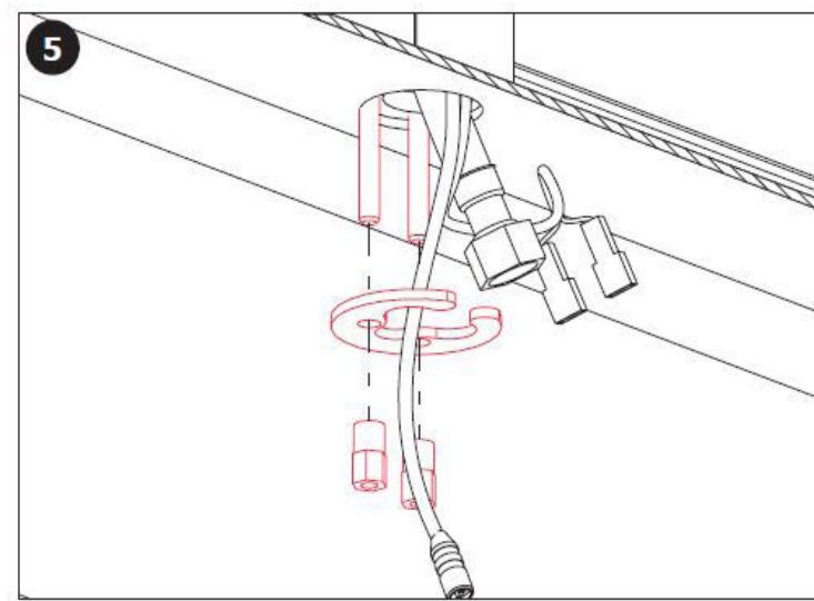
Fit mounting plate and hex nuts
