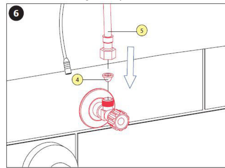
Fit filter into angle valve
